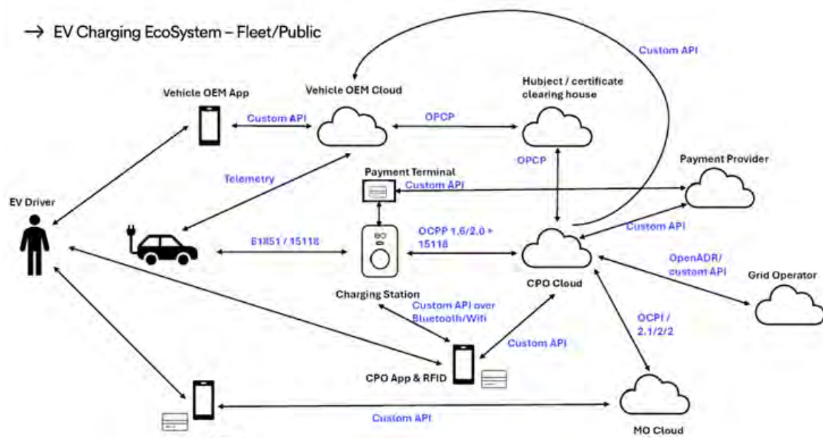
Fig 1: EV Charging Eco System Fleet/Public, Source: EO Charging
